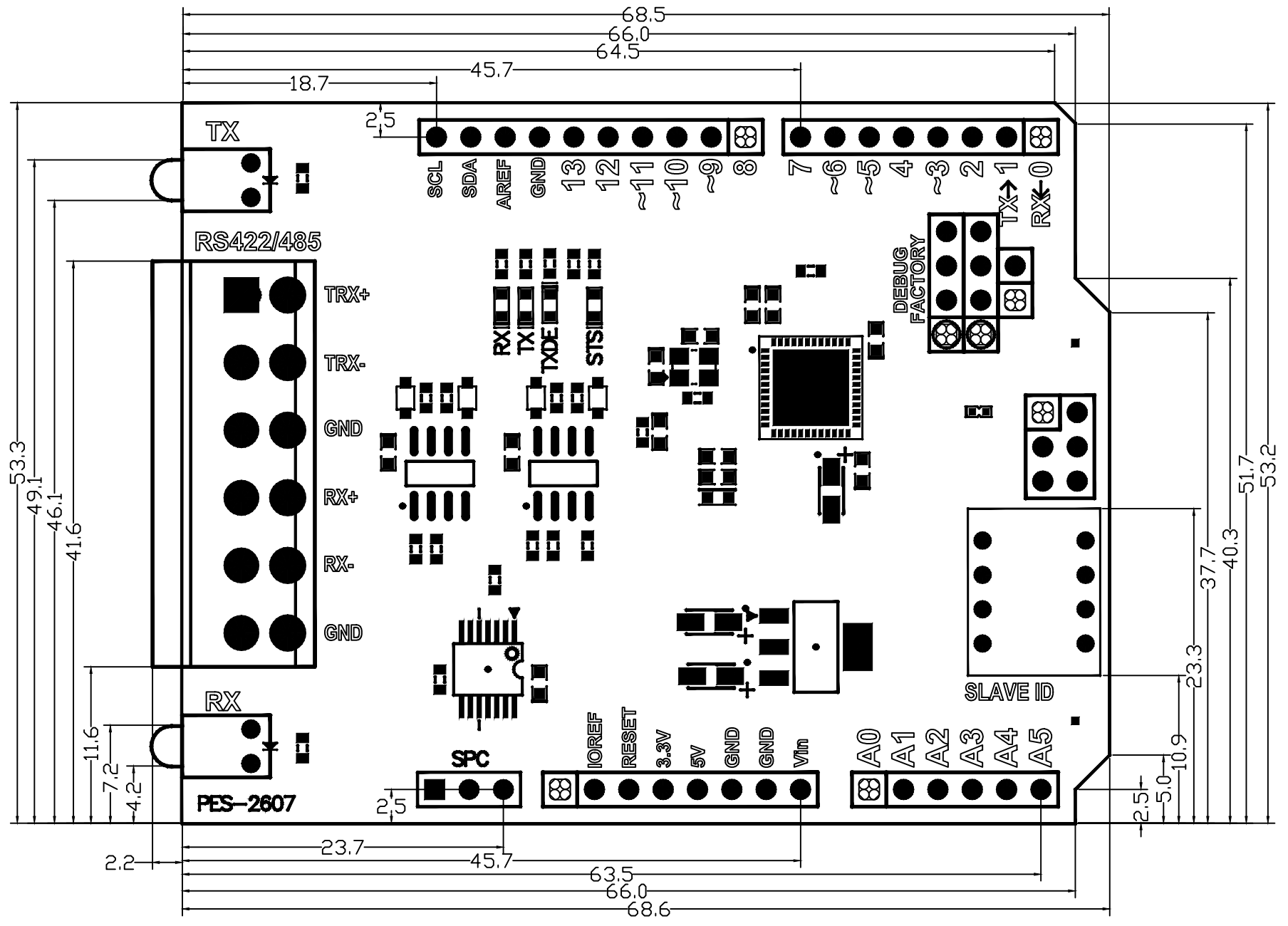
PES-2607 Dimension (mm)
